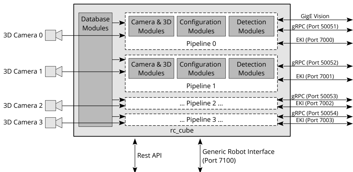
Fig. 5.1: Overview of the pipeline-specific and global software modules on the rc_cube
