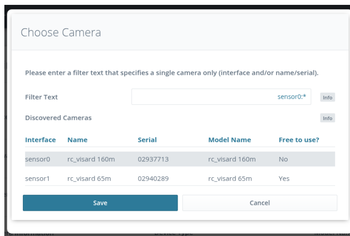
Fig. 4.4: Choosing the camera by setting a device filter
