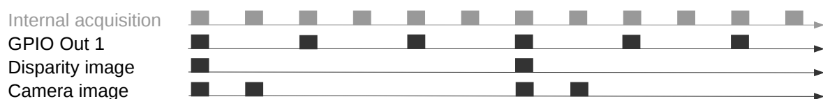
Fig. 5.36: Example of using the ExposureAlternateActive mode for GPIO Out 1 with a user-defined frame rate of 8 Hz. The internal image acquisition is always 25 Hz. GPIO Out 1 is HIGH for the exposure time of every second image. A disparity image is computed for images where Out 1 is HIGH and that are sent out via GigE Vision according to the user-defined frame rate. In ExposureAlternateActive mode, intensity images are always transmitted pairwise: one with GPIO Out 1 HIGH, for which a disparity image might be available, and one with GPIO Out 1 LOW.
