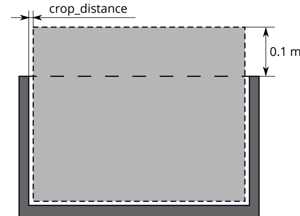
Fig. 5.38: Visualization of the inner volume of a load carrier. Only points which are inside this volume are considered for detections.
