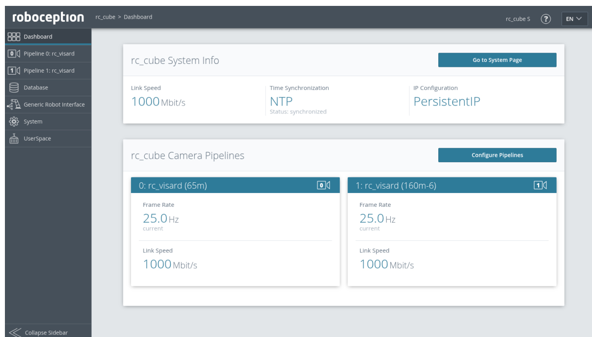
Fig. 6.1: Dashboard page of the rc_cube 's Web GUI
