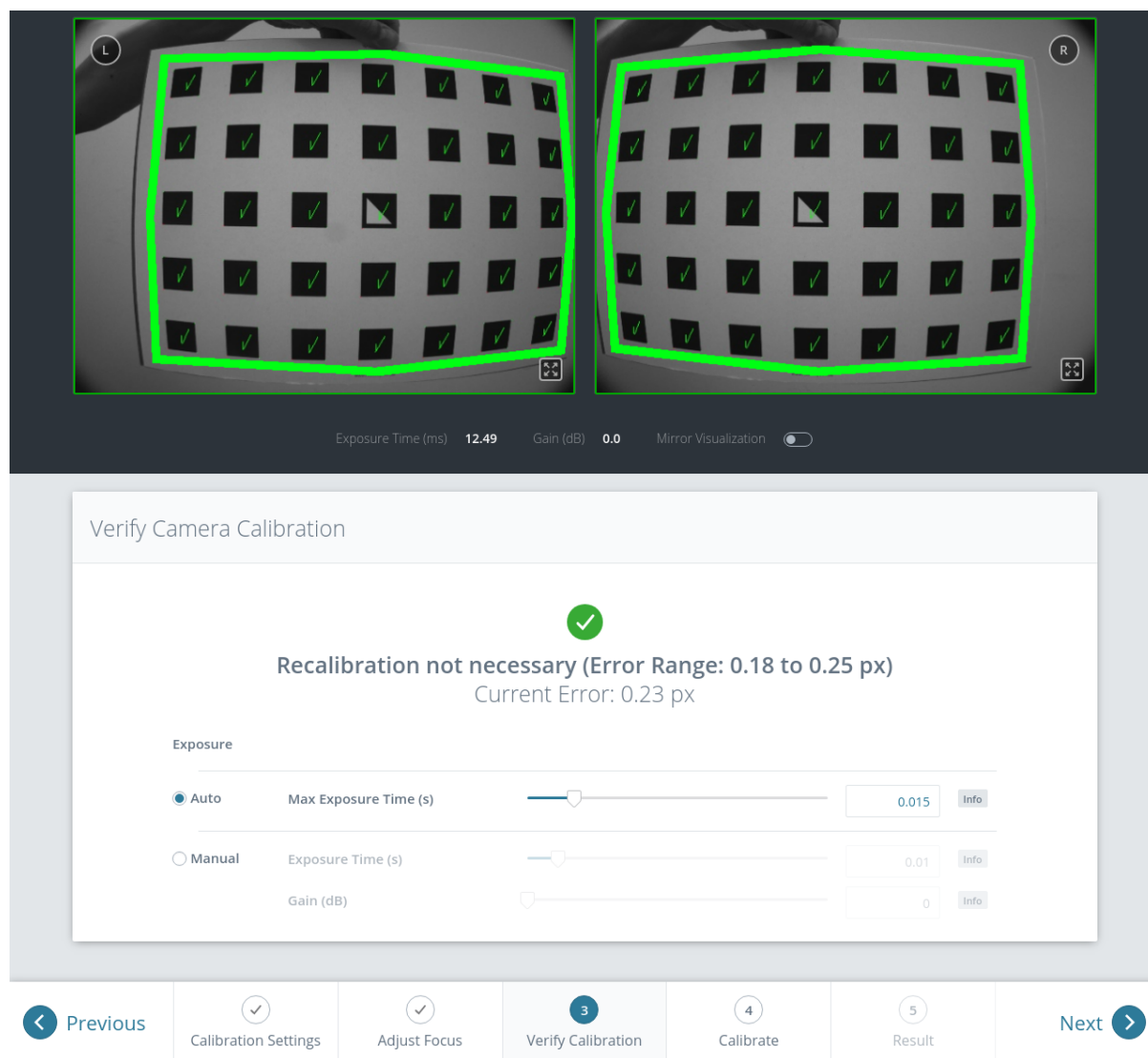
Fig. 5.29: Verification of calibration
