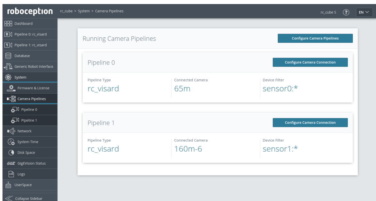
Fig. 4.1: Example of the Camera Pipelines page on an rc_cube with two running pipelines of type rc_visard
