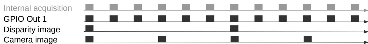
Fig. 5.35: Example of using the ExposureActive mode for GPIO Out 1 with a user-defined frame rate of 8 Hz. The internal image acquisition is always 25 Hz. GPIO Out 1 is HIGH for the exposure time of every image. A disparity image is computed for camera images that are sent out via GigE Vision according to the user-defined frame rate.
