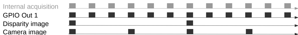
Fig. 6.34: Example of using the ExposureActive mode for GPIO Out 1 with a user-defined frame rate of 8 Hz. The internal image acquisition is always 25 Hz. GPIO Out 1 is HIGH for the exposure time of every image. A disparity image is computed for camera images that are sent out via GigE Vision according to the user-defined frame rate.
