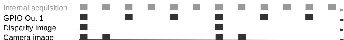
Fig. 6.36: Example of using the ExposureAlternateActive mode for GPIO Out 1 with a user-defined frame rate of 8 Hz. The internal image acquisition is always 25 Hz. GPIO Out 1 is HIGH for the exposure time of every second image. A disparity image is computed for images where Out 1 is HIGH and that are sent out via GigE Vision according to the user-defined frame rate. In ExposureAlternateActive mode, intensity images are always transmitted pairwise: one with GPIO Out 1 HIGH, for which a disparity image might be available, and one with GPIO Out 1 LOW.
