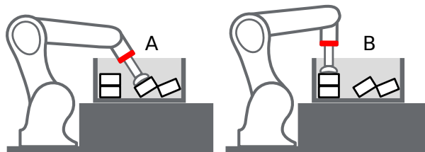
Fig. 6.42: Case A would be marked as collision only if check_flange is true, because the robot's flange (red) is inside the load carrier. Case B is collision free independent of check_flange .
