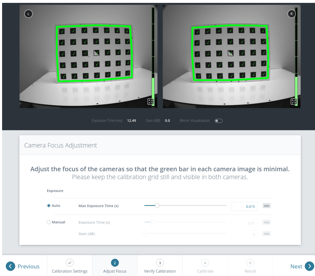
Fig. 6.29: Adjust the focus of each camera
