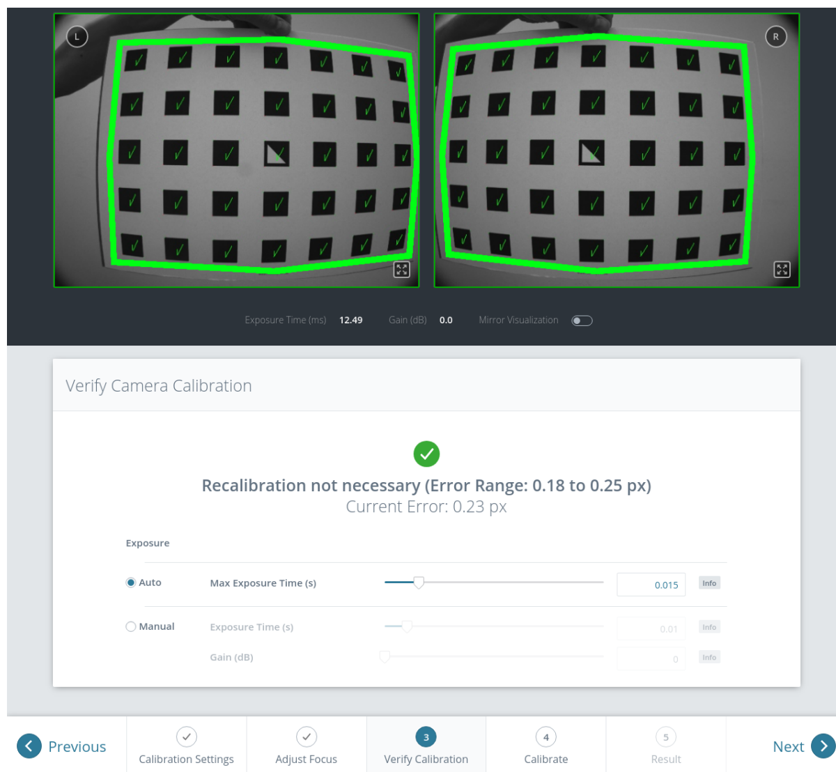
Fig. 6.30: Verification of calibration
