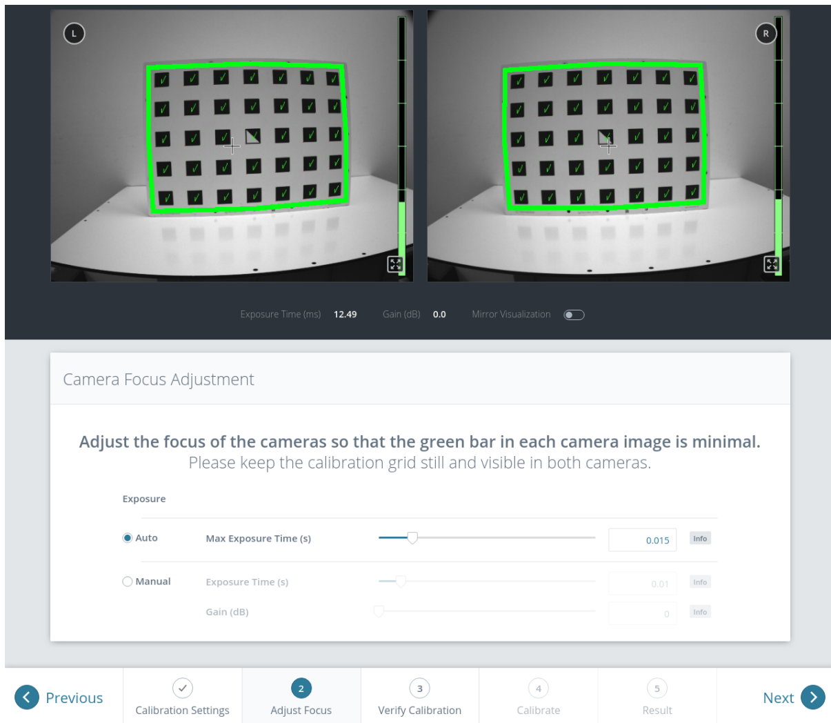
Fig. 6.28: Adjust the focus of each camera
