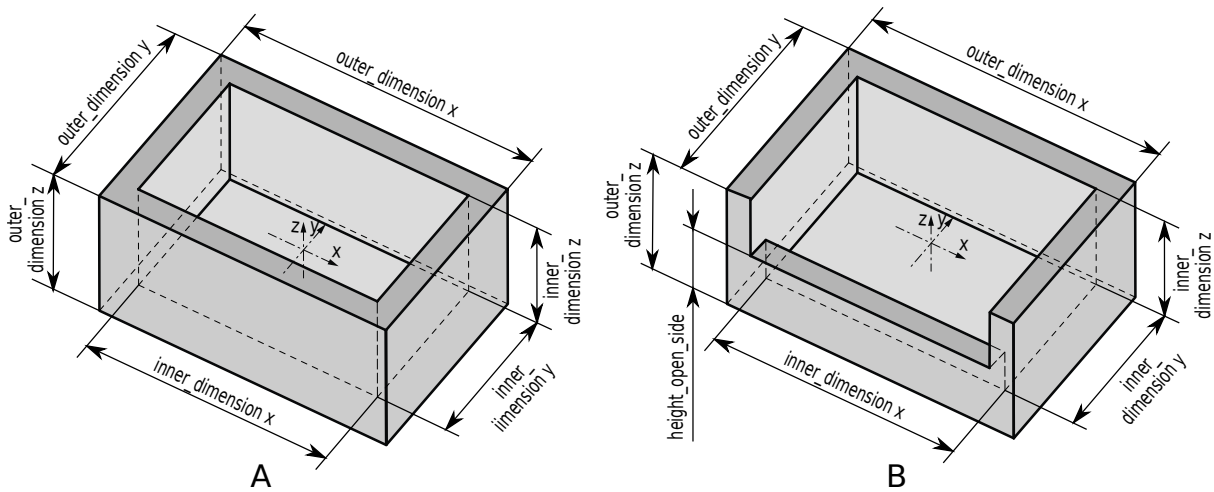
Fig. 6.41: Examples of a standard 4-sided load carrier (A) and a 3-sided load carrier (B)
