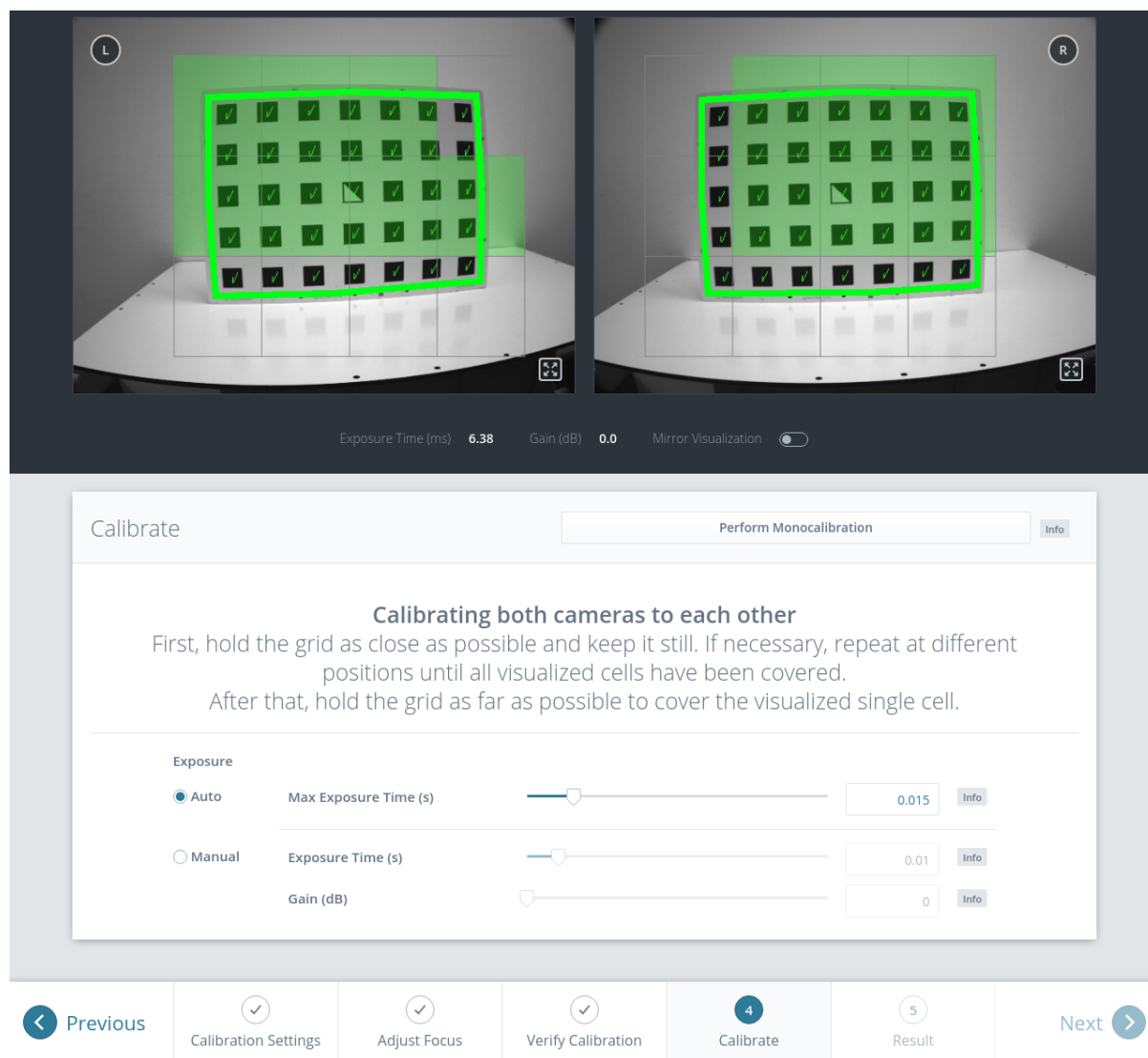
Fig. 6.32: Stereo calibration: Hold the grid as close as possible to fill all visualized cells
