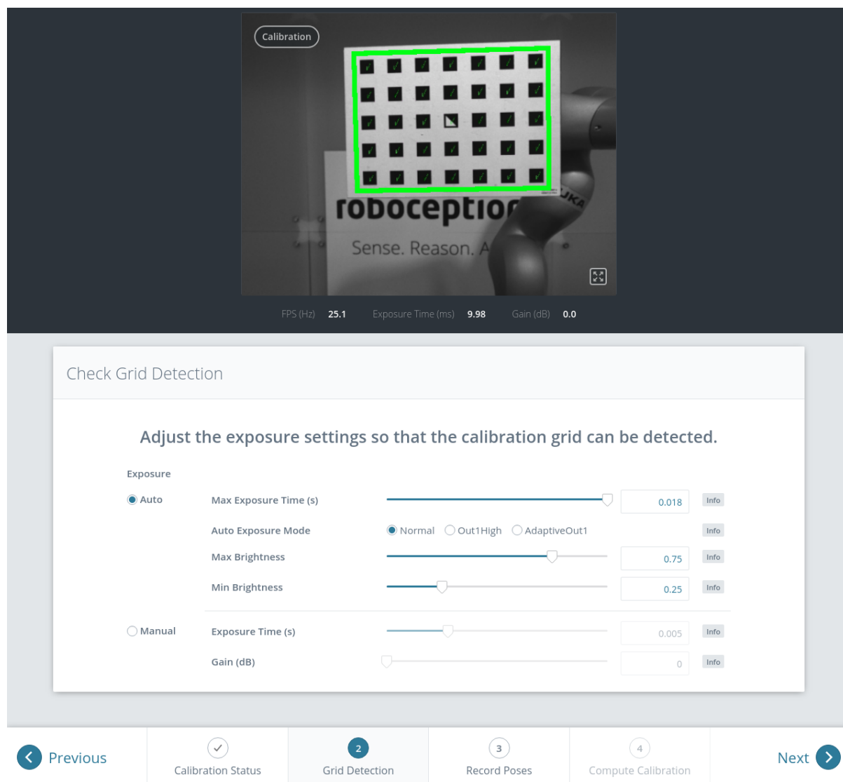
Fig. 6.22: Checking the calibration grid detection
