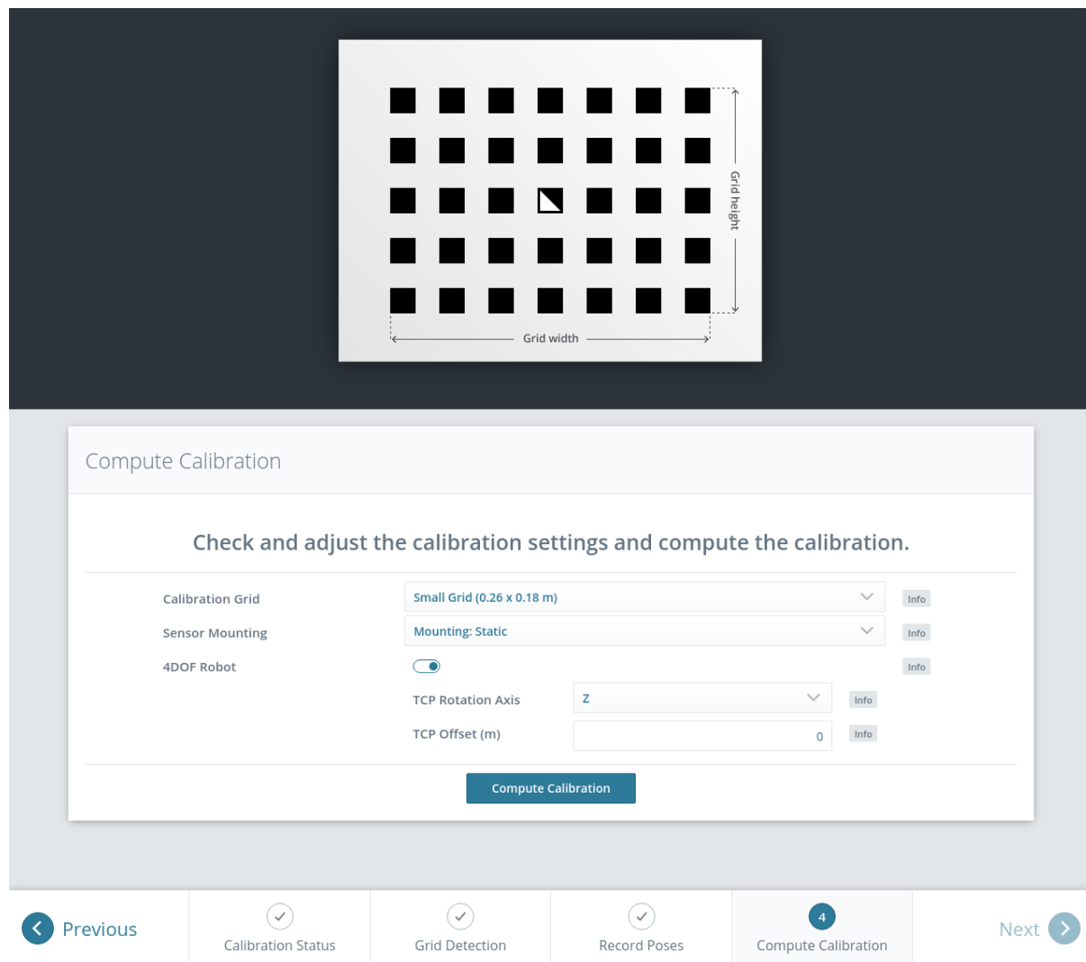
Fig. 6.26: Defining hand-eye calibration parameters and computing the calibration result via the rc_cube 's Web GUI
