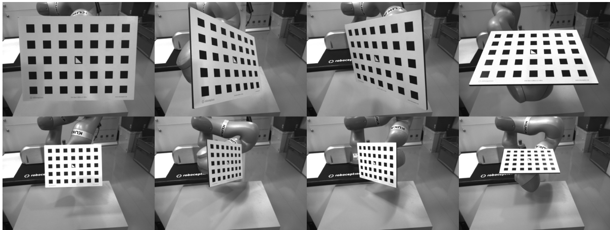
Fig. 6.25: Recorded camera images as input for the calibration procedure
