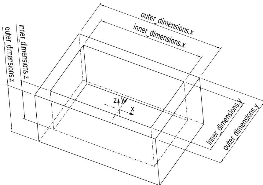
Fig. 6.38: Load carrier with reference frame and inner and outer dimensions
